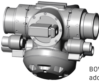
Bailout valve (BOV)
