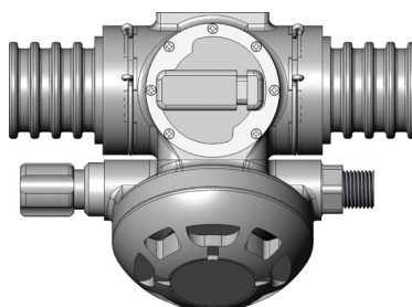
Hose nipples for Inspiration CCR
