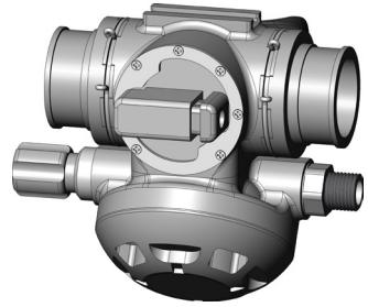
Bailout valve (BOV) with integrated Automatic diluent valve (ADV)
